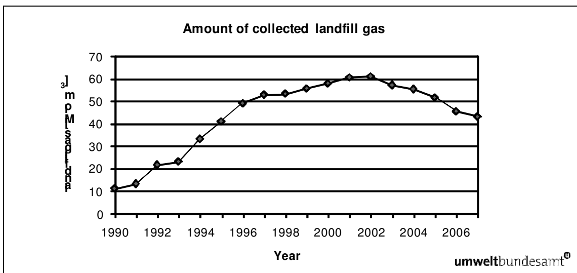
Figure 13: Amount of collected landfill gas 1990 to 2007 (ROLLAND & OLIVA 2004, SCHACHERMAYER & LAMPERT 2008).
