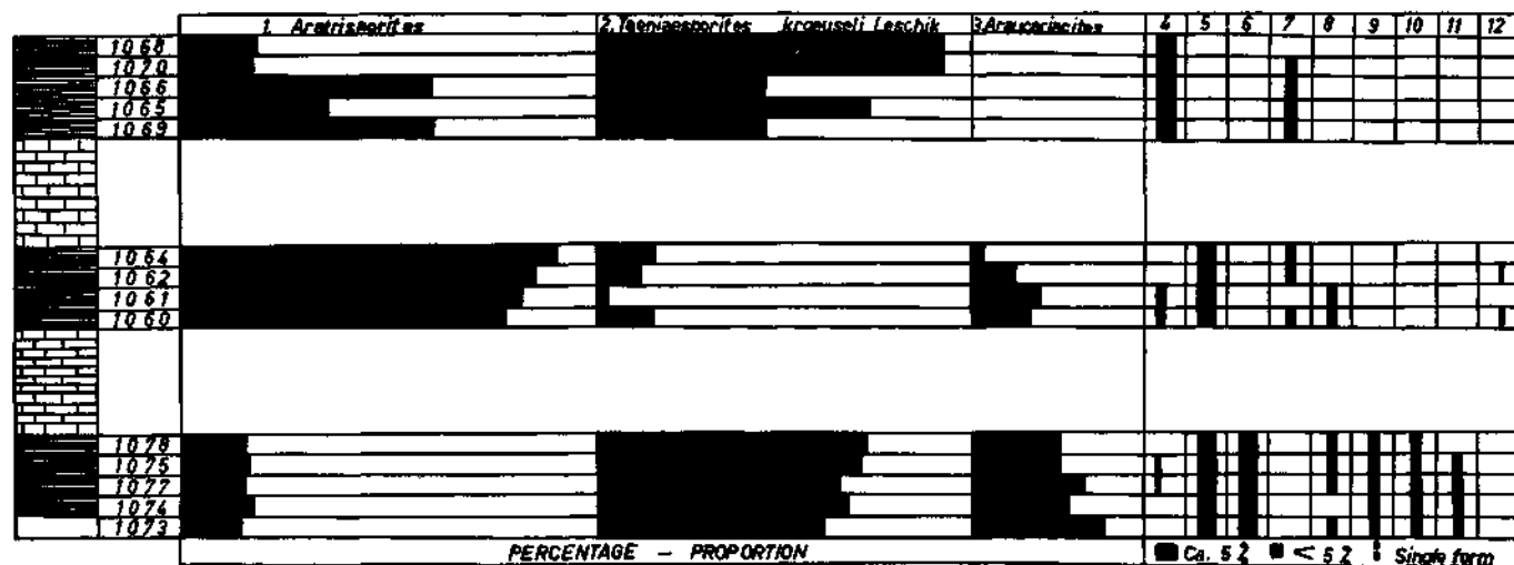
Text Fig. 3. 1. Aratrisporites, 2. Taeniaesporites kraeuseli Leschik, 3. Araucariacites, 4. Klausipollenites, 5. Cycadopites, 6. Decussatisporites spp., 7. Cycadopites aff. Marsupipollenites, 8. Rimaesporites, 9. Monosulcites cf. minimus Cookson, 10. Parvisaccites, 11. Leschikisporis aduncus (Leschik), 12. Zebrasporites.
