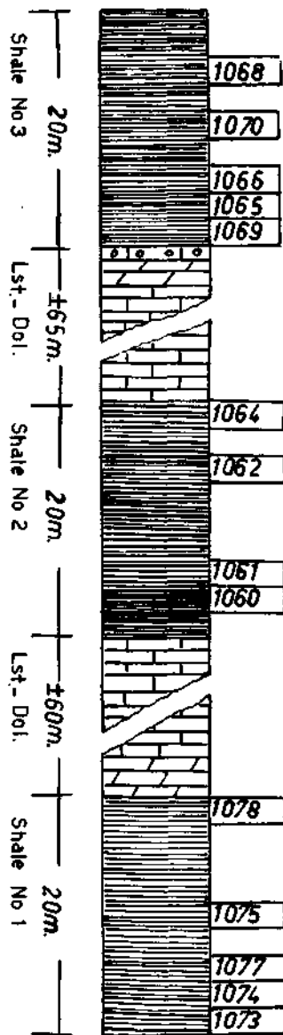
GENERALIZED LITHOLOGY INDICATING THE LOCATION OF SAMPLES
