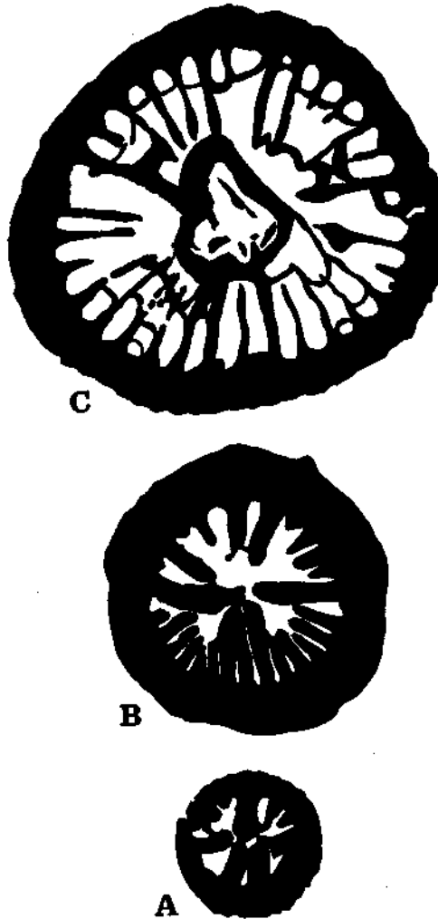
Abb. 8. Holotypus von Pentamplexus schindewolfi n. sp., Productus -Limestone, Loc. T 67—88, River 1 (MMH 11935). 4 X.
