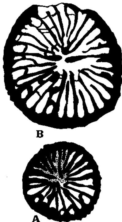
Abb. 11. Cryptophyllum ( Tachylasma? ) sp.?, Productus -Limestone, Loc. T 67—88, River F (MMH 11940). A, C 4,3 \times ; B 5 \times .
