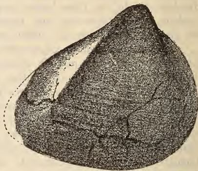
Myophoria truncata GF. sp. Oberer Stringocephalenkalk. Paffrath. Berliner Museum (Original KEFERSTEIN's).
