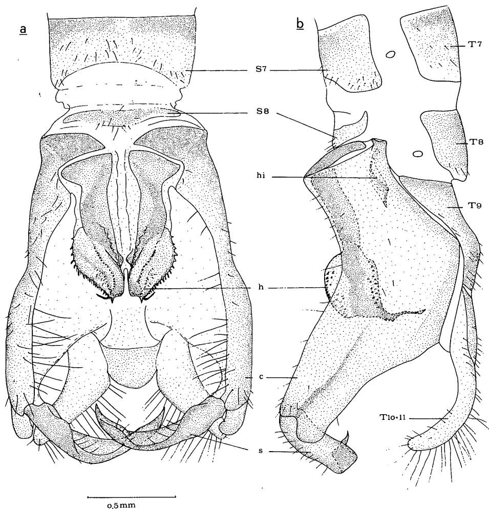
Abb. 2. Raphidia (Aliaberaphidia) tenochtitlana n.sp., ♂. – Genitalsegmente, ventral (a) und lateral (b). – c = 9. Koxopodit, h = Hypovalva, hi = Hypandrium internum, s = Stylus, S = Sternite, T = Tergite.
