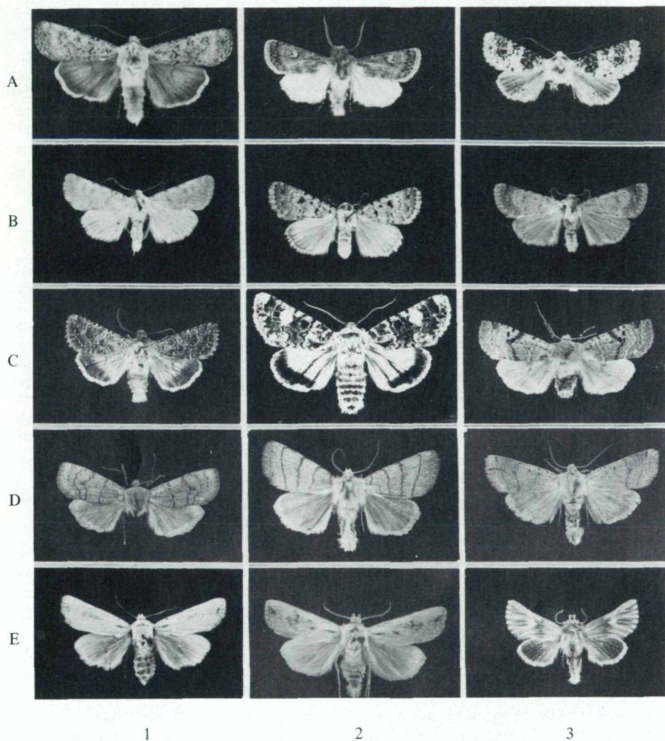
A 1: Euxoa (Chorizagrotis) friedeli n.sp., ♂, Gürün. – A 2: Euxoa rubrior n.sp., ♂, Gürün. – A 3: Hadena cavalla n.sp., ♂, Gürün. – B 1: Caradrina (Eremodrina) avis n.sp., ♂, Gürün. – B 2: Caradrina (Eremodrina) conditorana n.sp., ♂, Gürün. – B 3: Caradrina (Eremodrina) inumbratella n.sp., ♂, Gürün. – C 1: Discestra pugnax intermedia n.ssp. (bona species?), ♂, Gürün. – C 2: Oxytripia noctivolans n.sp., ♂, Gürün. – C 3: Conistra asiatica n.sp., ♂, Kızılcahamam. – D 1: Conistra (Dasycampa) ragusae archaia n.ssp., ♂, Kızılcahamam. – D 2: Charanyca trigrammica asiaminorica n.ssp., ♂, Kızılcahamam. – D 3: Agrochola humilis anatolica n.ssp., ♂, Kızılcahamam. – E 1: Agrotis endogaea punica n.ssp., ♀, Hammamet. – E 2: Agrotis endogaea punica n.ssp., ♂, Hammamet. – E 3: Copiphana olivina pseudoliva n.ssp., ♂, Gürün.
