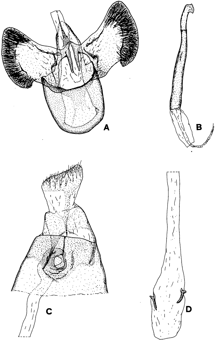
PLATE III. A - D: Aspilapteryx tringipennella Z. A: Male genitalia; B: Aedoeagus; C: Female genitalia; D: Bursa copulatrix.
