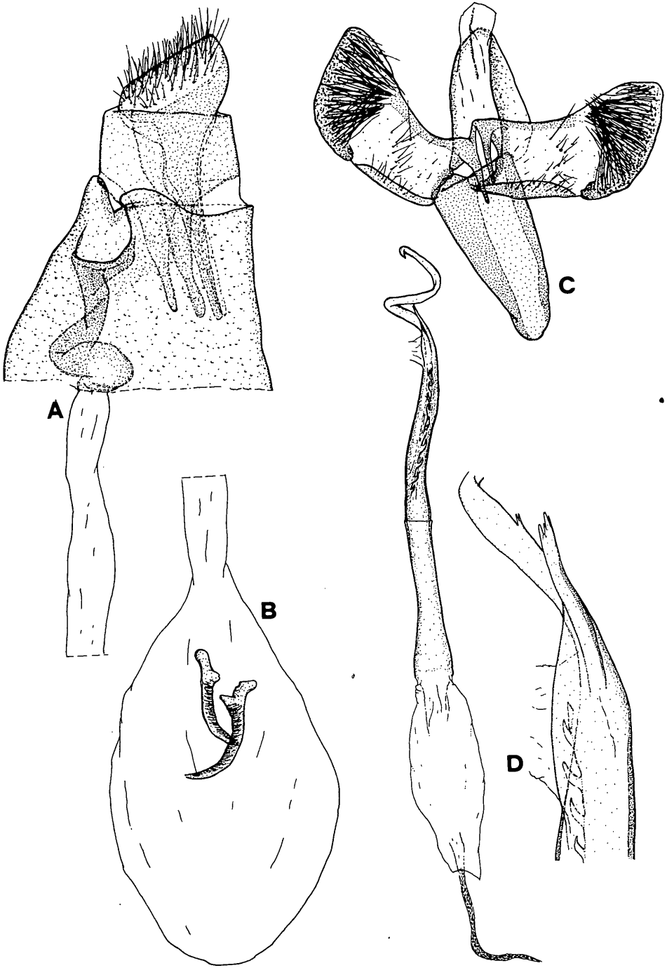
PLATE IV. A-D: Aspilapteryx multipunctella CHRÉT. A: Female genitalia; B: Bursa copulatrix; C: Male genitalia; D: Aedoeagus.
