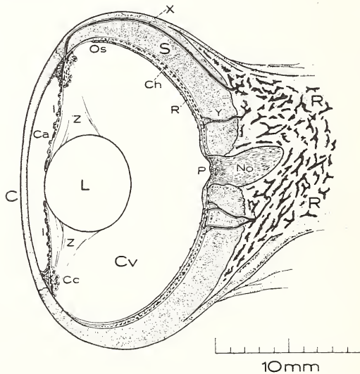
Abb. 2. Horizontalschnitt durch das Auge von Delphinapterus leucas . C = Cornea; Ca = Camera anterior; Cc = Corpus ciliare; Ch = Choroidea; Cv = Corpus vitreum; I = Iris; L = Lens; No = Nervus opticus; P = Papilla nervi optici; R = Retina. (Nach PILLERI 1963)
