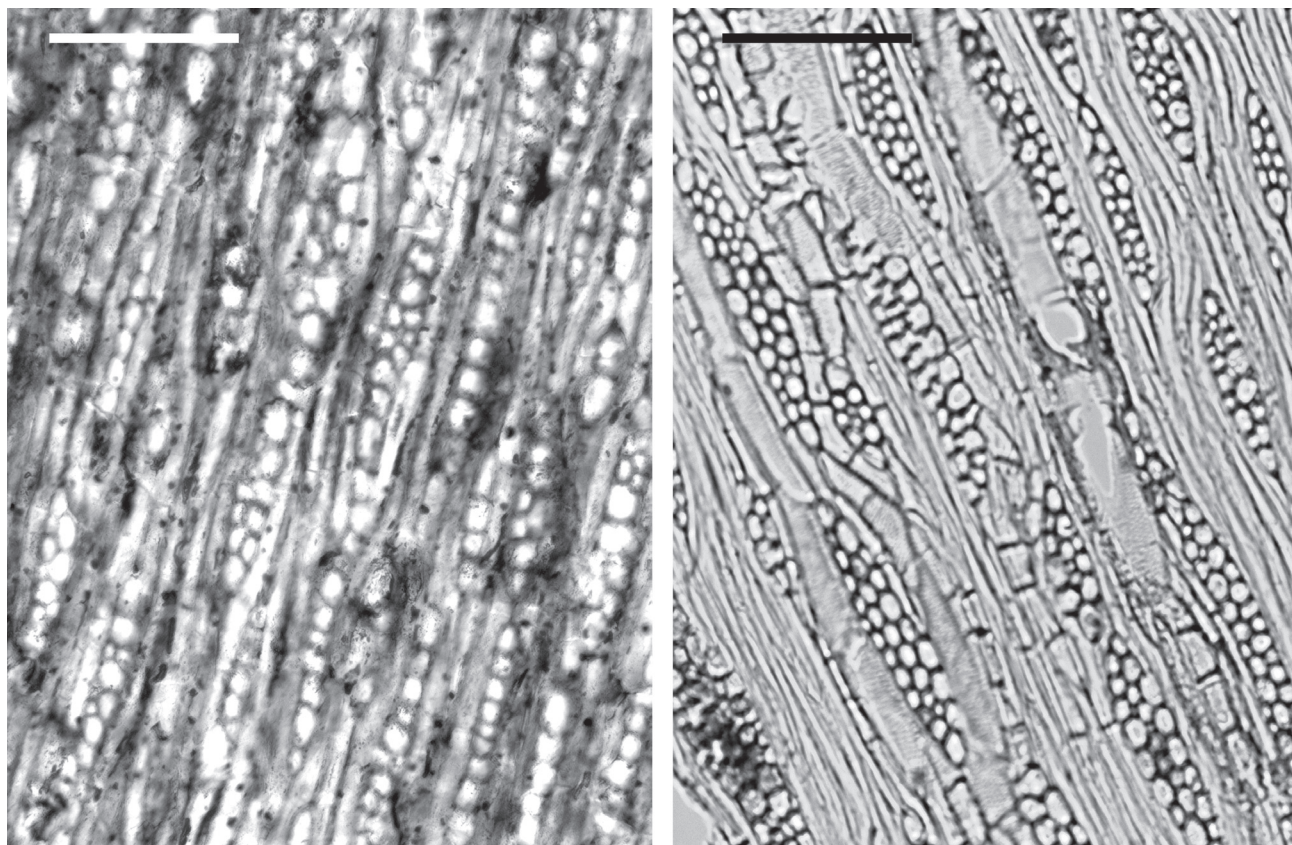
Textfigure 6: Capparidoxylon holleisii nov. sp. (left, BSPG 2004 XV 1), and Capparis speciosa (right, RAKF No.3223). Note the similarities in cellular composition of the rays; scale bars = 200 µm, x 115.
