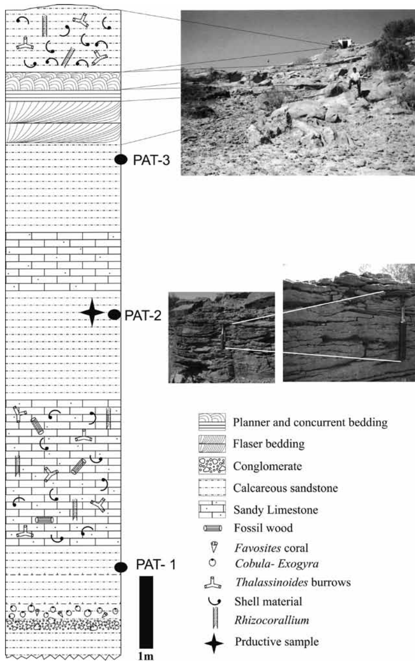
Textfigure 3: Sampling location from the middle part of the Dingi Hill Member of the Kaladongar Formation exposed at the Point 16 hillock (23° 59' 40" N: 69° 42' 28" E) at Kuar Bet in the Pachchham Island.
