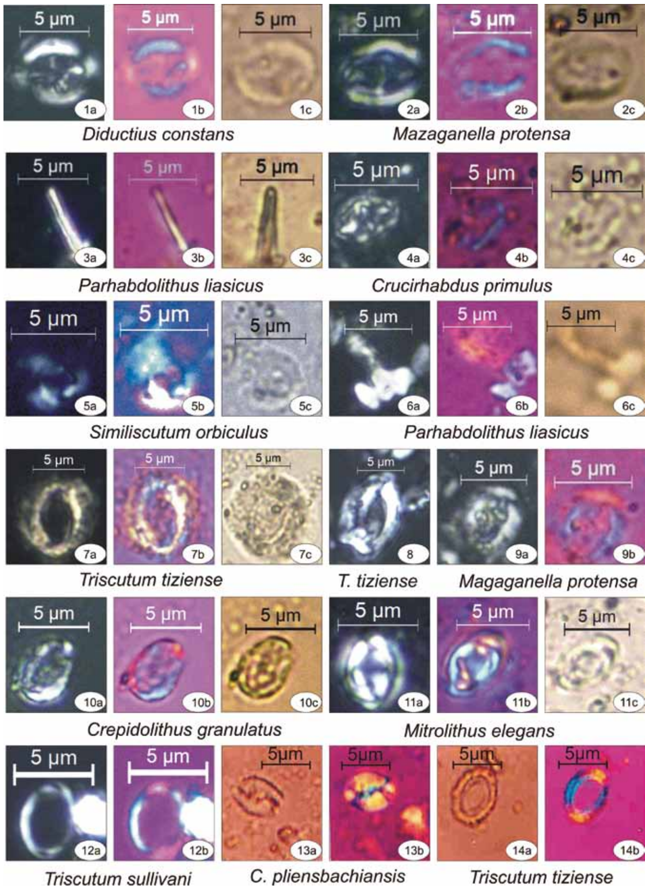
Plate 4: Pliensbachian-Toarcian age reworked nannofossils from Wagad (1–4), Jumara (5–11), Habo (12) and Jara (13–14) domes (Kachchh).
