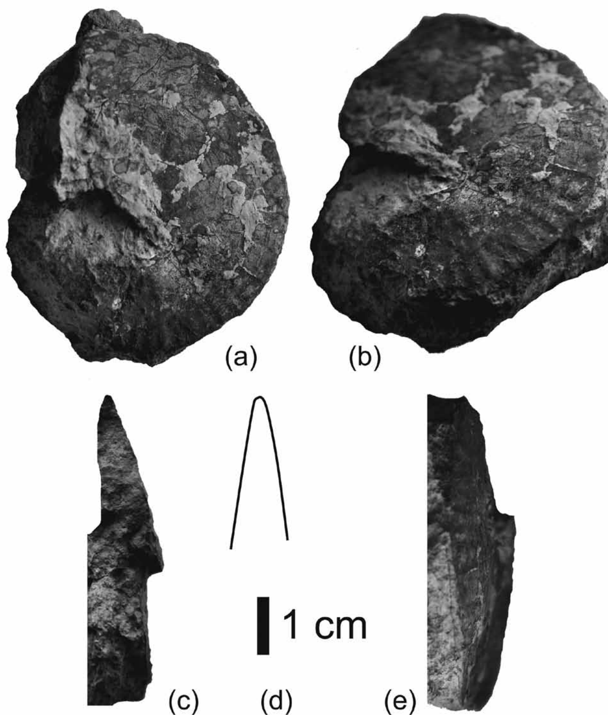
Figure 8: (a–e) Micromphalites ( Clydomphalites ) clydocromphalus Arkell [M], specimen no. SJ/Ju/14/A4/1, Yellow Bed (bed A4), Jumara Dome. (a): Lateral view. (b): Lateral view at an angle to highlight ribbing pattern. (c): Apertural view. (d): Whorl-section reconstructed from (c). (e): Ventral view showing the narrow keel.
