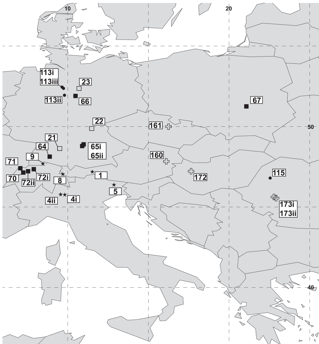
Figure 7: Pterosaur localities from the Upper Triassic to Upper Cretaceous of central and eastern Europe, including Germany, Italy, Austria, Switzerland, Poland, Romania, Hungary and the Czech Republic. Note that no Middle Jurassic pterosaur localities are currently known from these regions. Key: filled star, Upper Triassic; open squares, Lower Jurassic localities; filled squares, Upper Jurassic localities; filled circles, Lower Cretaceous localities; open crosses, Upper Cretaceous localities. Numbers in boxes refer to numbered localities in the text; other numbers refer to latitude and longitude.
