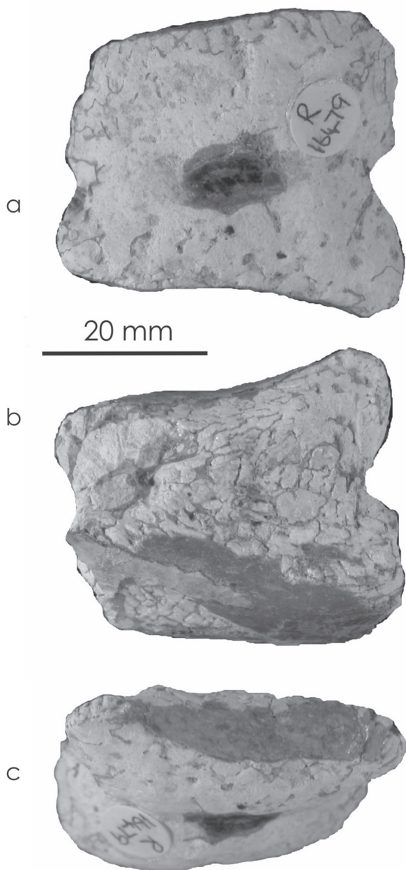
Figure 7: Partial, presumed cervical vertebra of an indeterminate ornithocheiroid pterosaur, BMNH R 16479c, from the White Chalk Formation of St Margaret's Bay, East Kent. a. highly eroded left lateral aspect. b. slightly oblique right lateral aspect. c. dorsal view.
