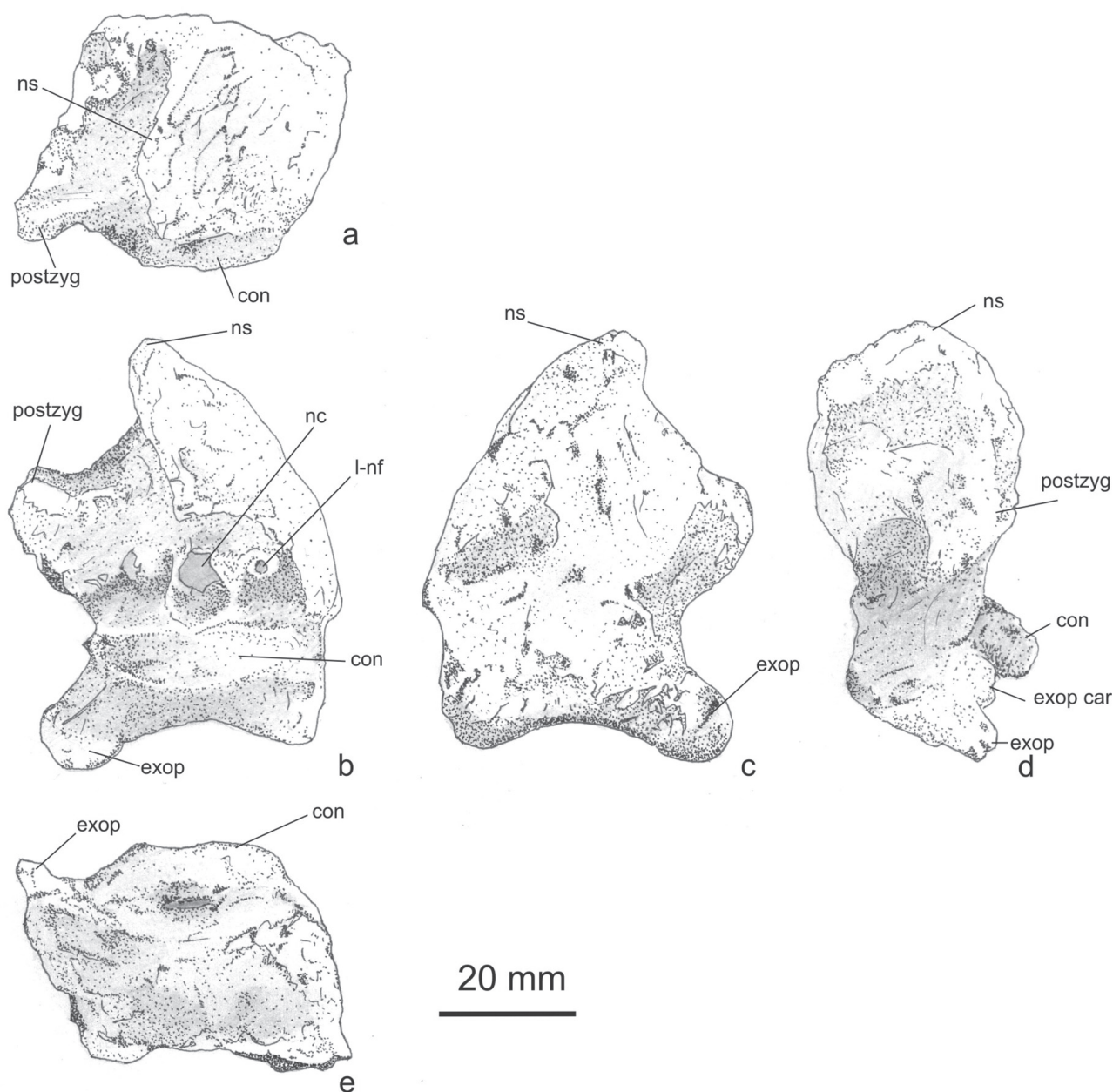
Figure 6: Drawings of indeterminate azhdarchoid mid cervical vertebra BMNH R 16479b. a, dorsal view; b, caudal view; c, cranial view; d, left lateral view; e, ventral view. For abbreviations see Figure 4.
