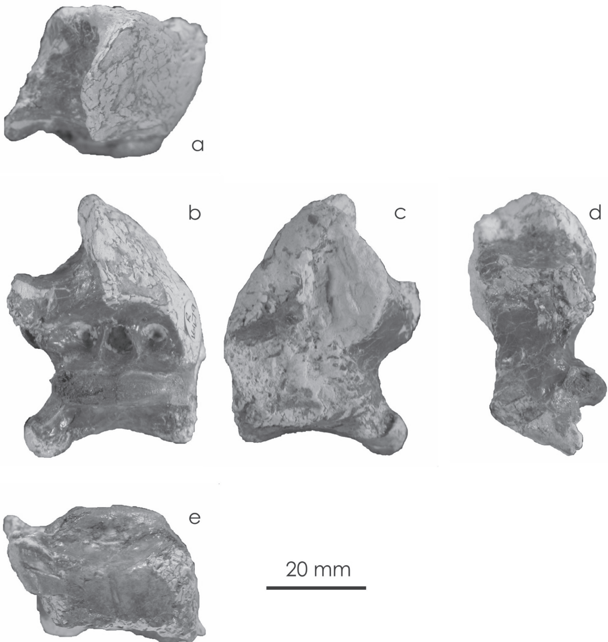
Figure 5: Mid cervical vertebra of an indeterminate ornithocheiroid pterosaur, BMNH R 16479b, from the White Chalk Formation of St Margaret's Bay, East Kent. a, dorsal aspect. b, caudal aspect. c, cranial aspect. d, right lateral aspect.
