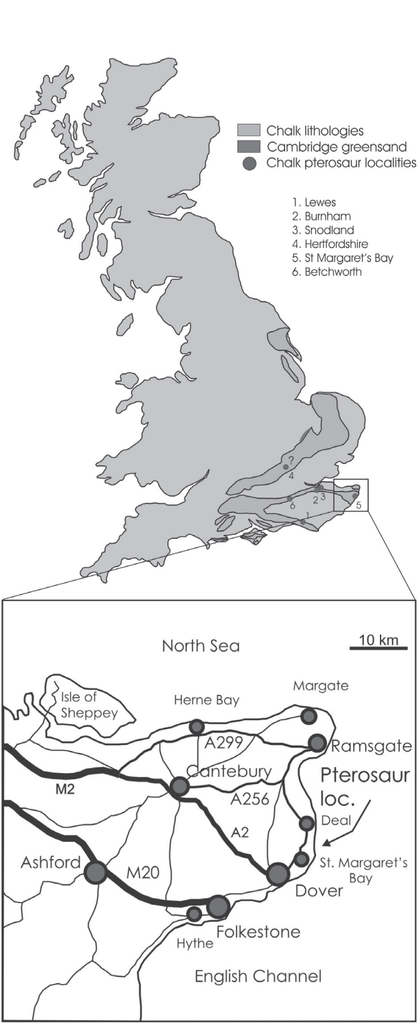
Figure 1: Location of English Chalk pterosaur localities and the locality of the pterosaur cervical vertebrae BMNH R16479a-c from the Coniacian of Kent, southern England.
