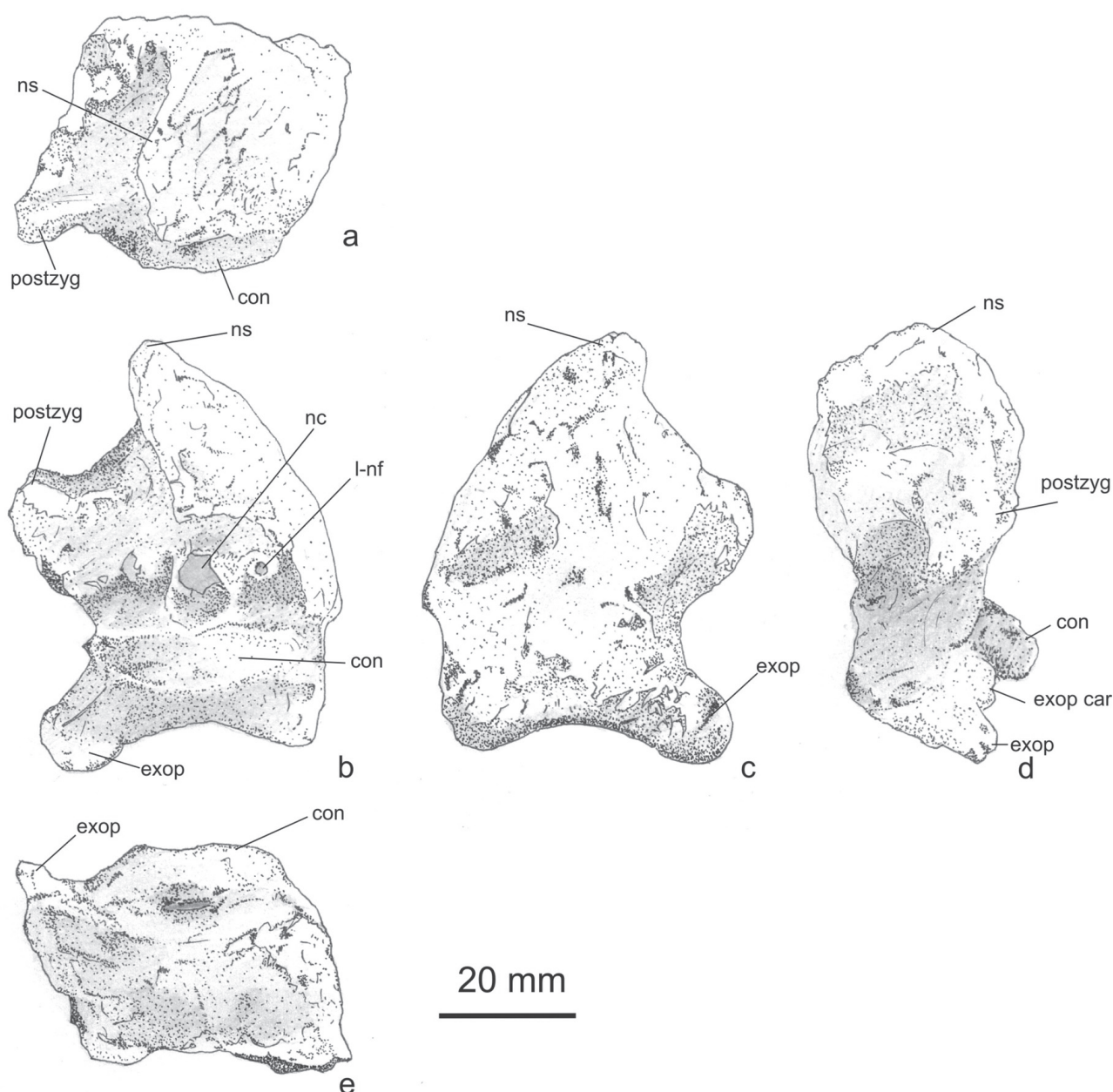
Figure 6: Drawings of indeterminate azhdarchoid mid cervical vertebra BMNH R 16479b. a , dorsal view; b , caudal view; c , cranial view; d , left lateral view; e , ventral view. For abbreviations see Figure 4.
