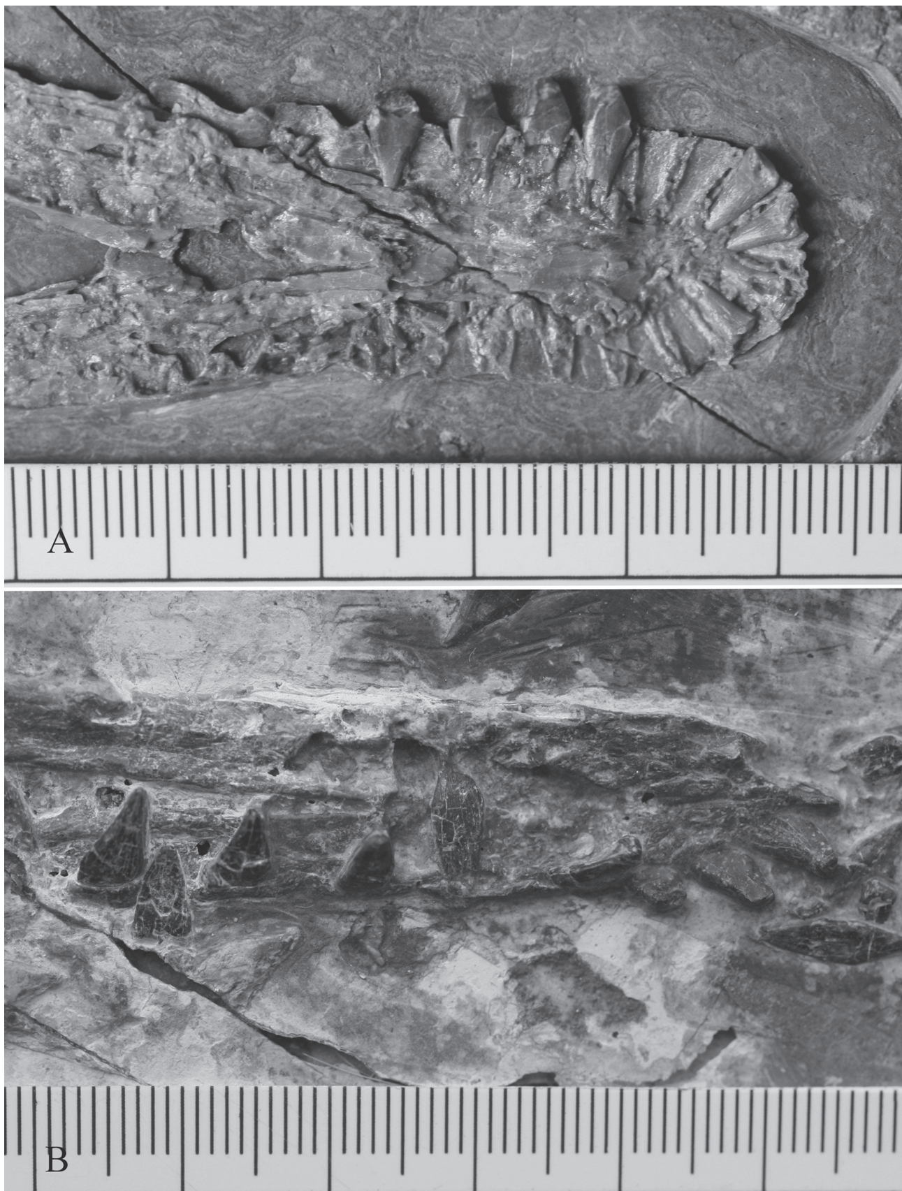
Figure 2: Rostral end comparisons of the lower jaws of Liaoxipterus brachyognathus (A), and Longchengpterus zhaoi (B). Scale bars are in centimeters.
