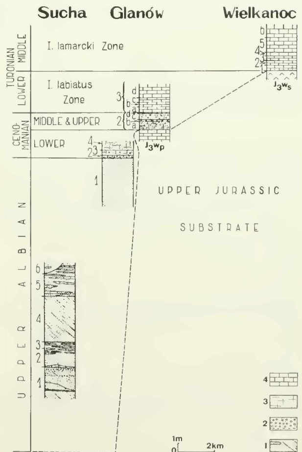
Fig. 3. Relation of the mid-Cretaceous transgressive sequence to the Upper Jurassic substrate (batten – J_3ws or platy limestones – J_3wp ; numbers of beds the same as in MARCINOWSKI 1974) near Glanów (cf. fig. 4 and pl. 1A–D) and neighbouring locality Sucha (cf. pl. 2, Figs. 2a–b) in the Polish Jura.
