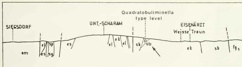
Fig. 2: Geological section 1:25 000 between the sedimentologic-tectonic units from Flysch (fg 1 ) to molasse (om) in the region of Eisenärzt and Siegsdorf indicating the tectonic position of the Danian level of Grub (p) (after GANSS 1956, modified). Arrow points to Bucheck locality encountered to the south of the Quadratobuliminella type locality (p). For abbreviations see also DE KLASZ & DE KLASZ, 1990: fig. 4.
