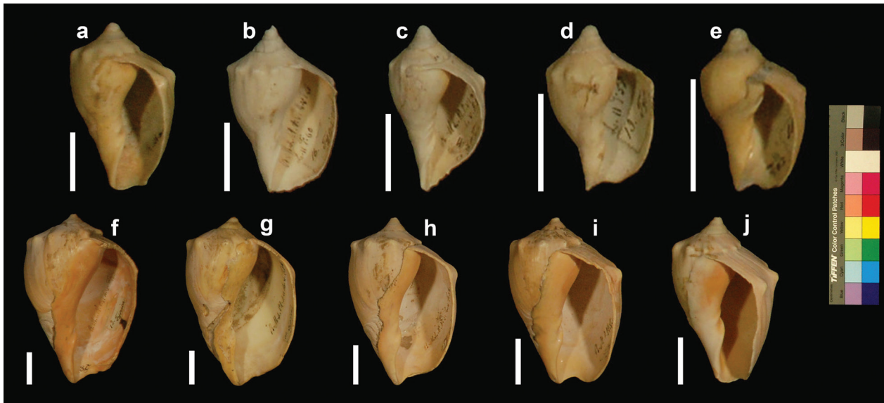
Figure 28. Voluta colocyntthis typica , specimens figured by Lahille (1895). See references on Table 10. Scale bars: 3 cm.
