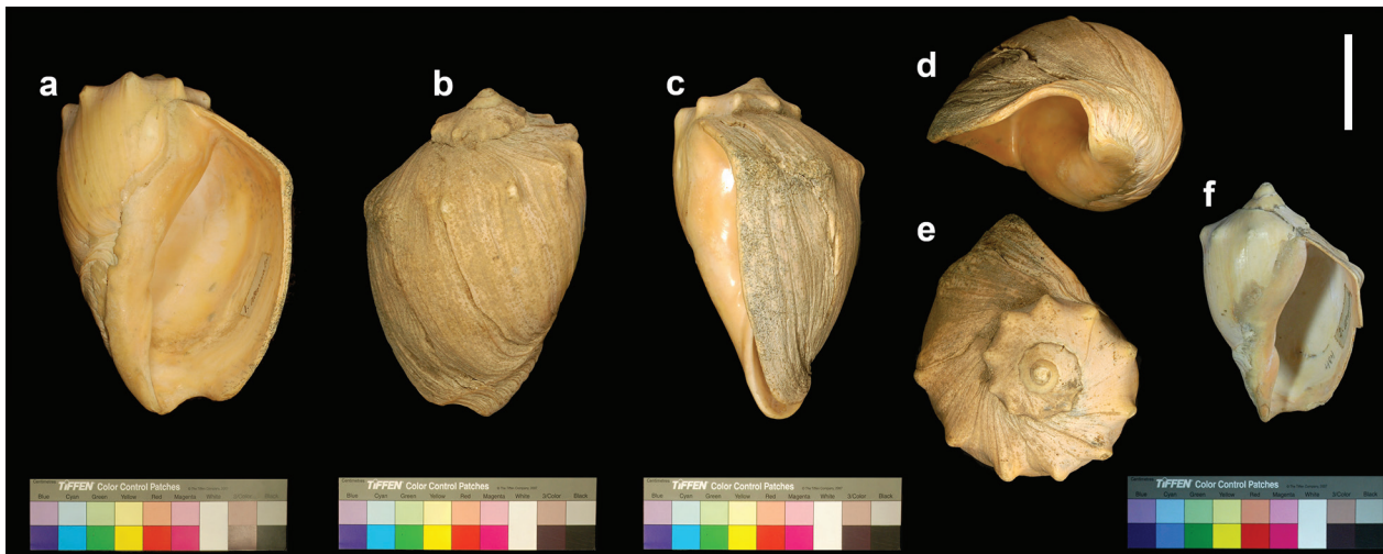
Figure 29. Voluta colocyntthis alternata , specimens not figured by Lahille (1895). a–e Specimen 1 a Apertural view b Dorsal view c Lateral view d Umbilical view e Apical view f Apertural view of specimen 2. Scale bar: 5 cm.
