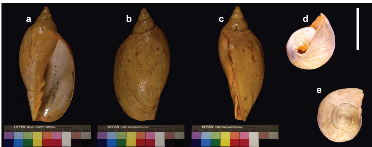
Figure 48. Voluta paradoxa typica specimen figured by Lahille (1895: pl. II, fig. 76b; pl. VIII, fig. 161; pl. XII, fig. 20) a Apertural view b Dorsal view c Lateral view d Umbilical view e Apical view. Scale bar: 5 cm.
