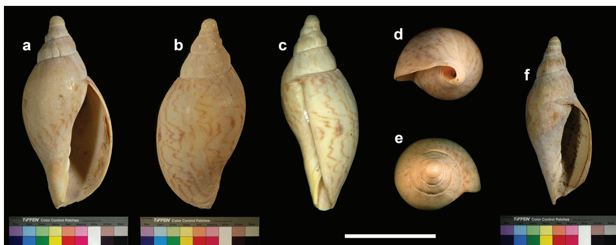
Figure 3. Voluta ambigua constricta . a–e Specimen figured by Lahille (1895: pl. VIII, fig. 164) a Apertural view b Dorsal view c Lateral view d Umbilical view e Apical view f Specimen figured by Lahille (1895, pl. VIII, fig. 163) in apertural view. Scale bar: 3 cm.
