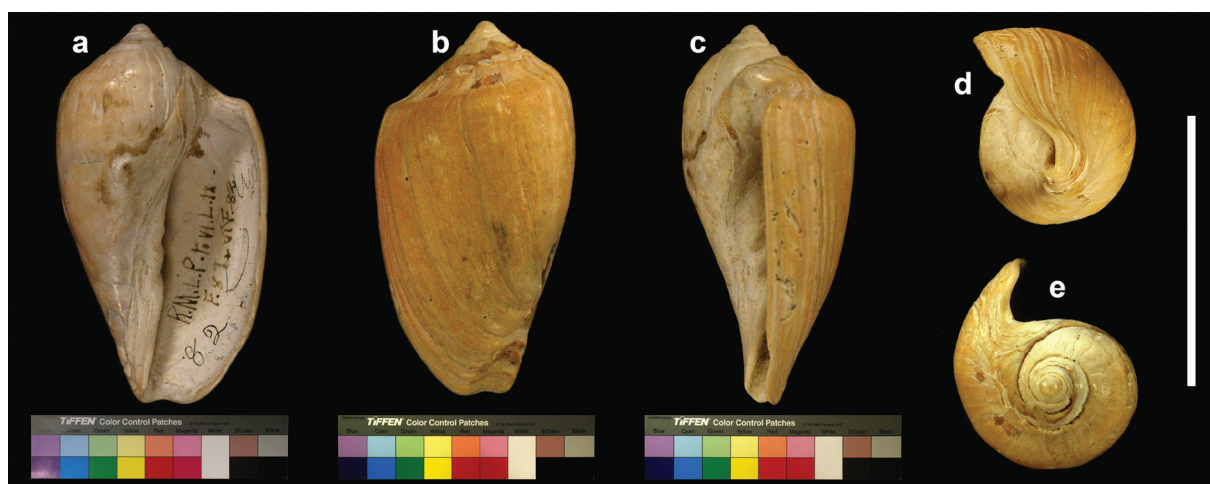
Figure 22. Voluta angulata mixta , specimen figured by Lahille (1895: pl. IX, fig. 8; pl. VI, fig. 82). a Apertural view b Dorsal view c Lateral view d Umbilical view e Apical view. Scale bar: 5 cm.
