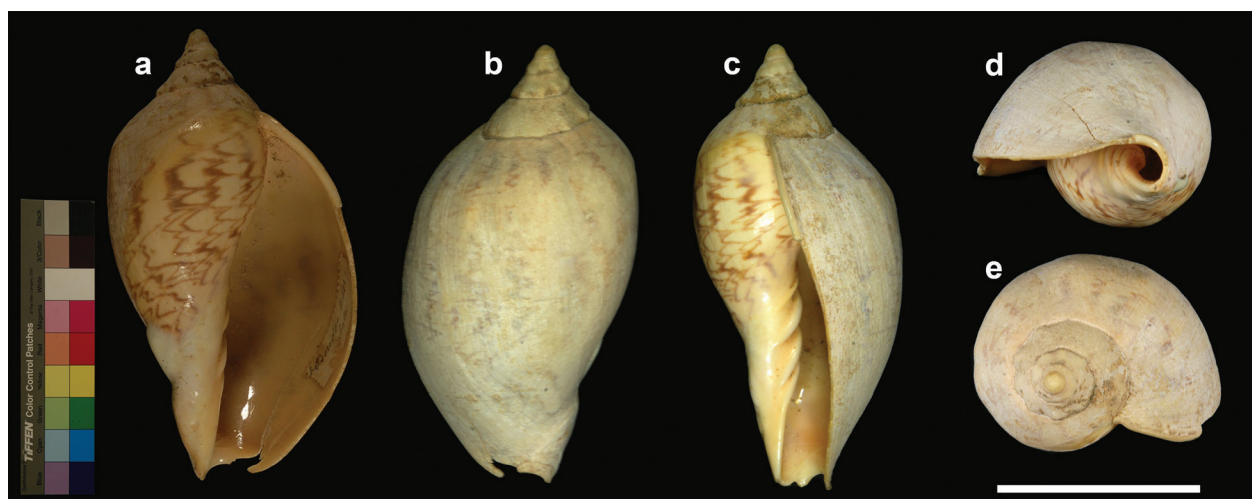
Figure 4. Voluta ambigua pseudotuberculata , holotype figured by Lahille (1895: pl. XI, fig. 6) a Apertural view b Dorsal view c Lateral view d Umbilical view e Apical view. Scale bar: 5 cm.
