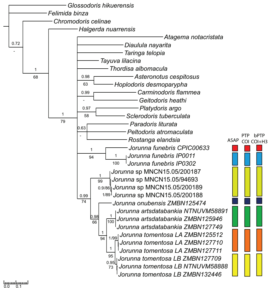
Figure 6. Bayesian inference tree based on the concatenate sequence dataset (COI+H3) collapsed (PP < 0.5). Numbers at the top of nodes indicate Bayesian Posterior probability (PP) and on the bottom bootstrap support from the maximum likelihood analysis (BS). Colored bars on the right represent the results of the species delimitation analyses on the Jorunna spp., from left to right: ASAP on COI dataset, PTP on COI dataset, bPTP on COI+H3 dataset.
